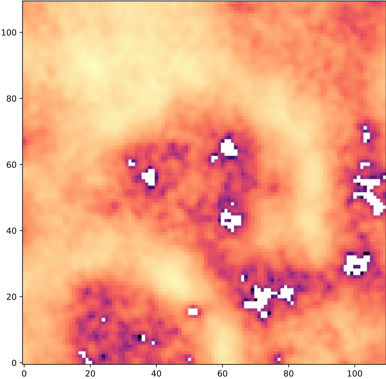
Region: 7 HI - Type 1
