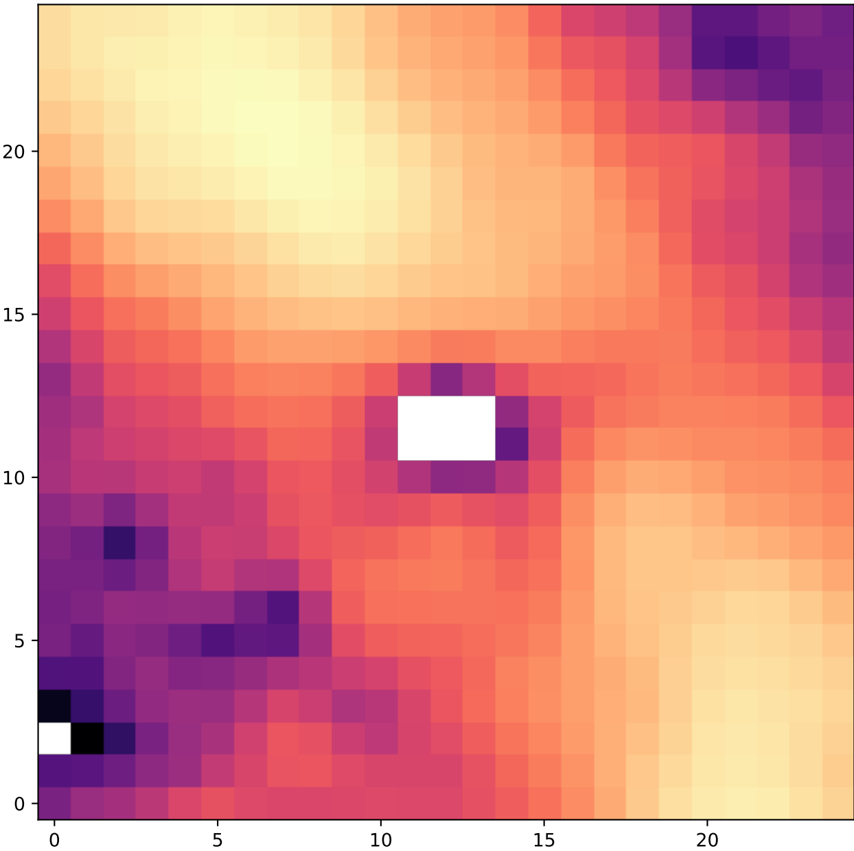
Region: 8 HI - Type 2
