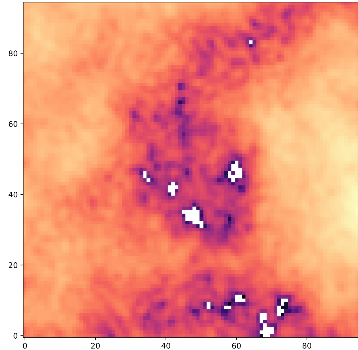
Region: 16 HI - Type 1
