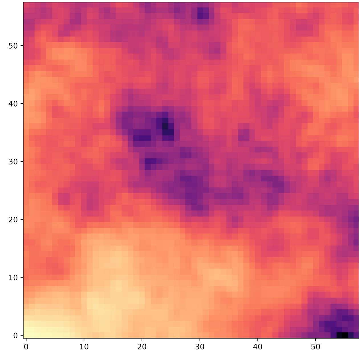
Region: 15 HI - Type 1
