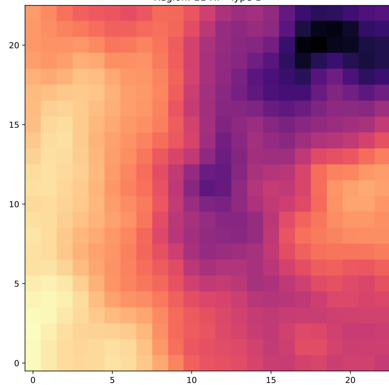
Region: 11 HI - Type 1
