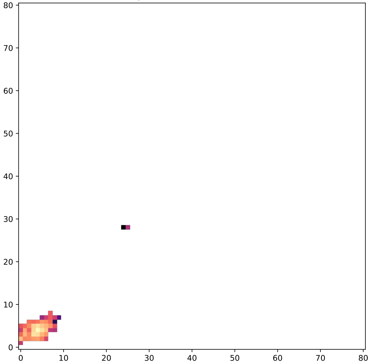
H-alpha - Classification: Diffuse
