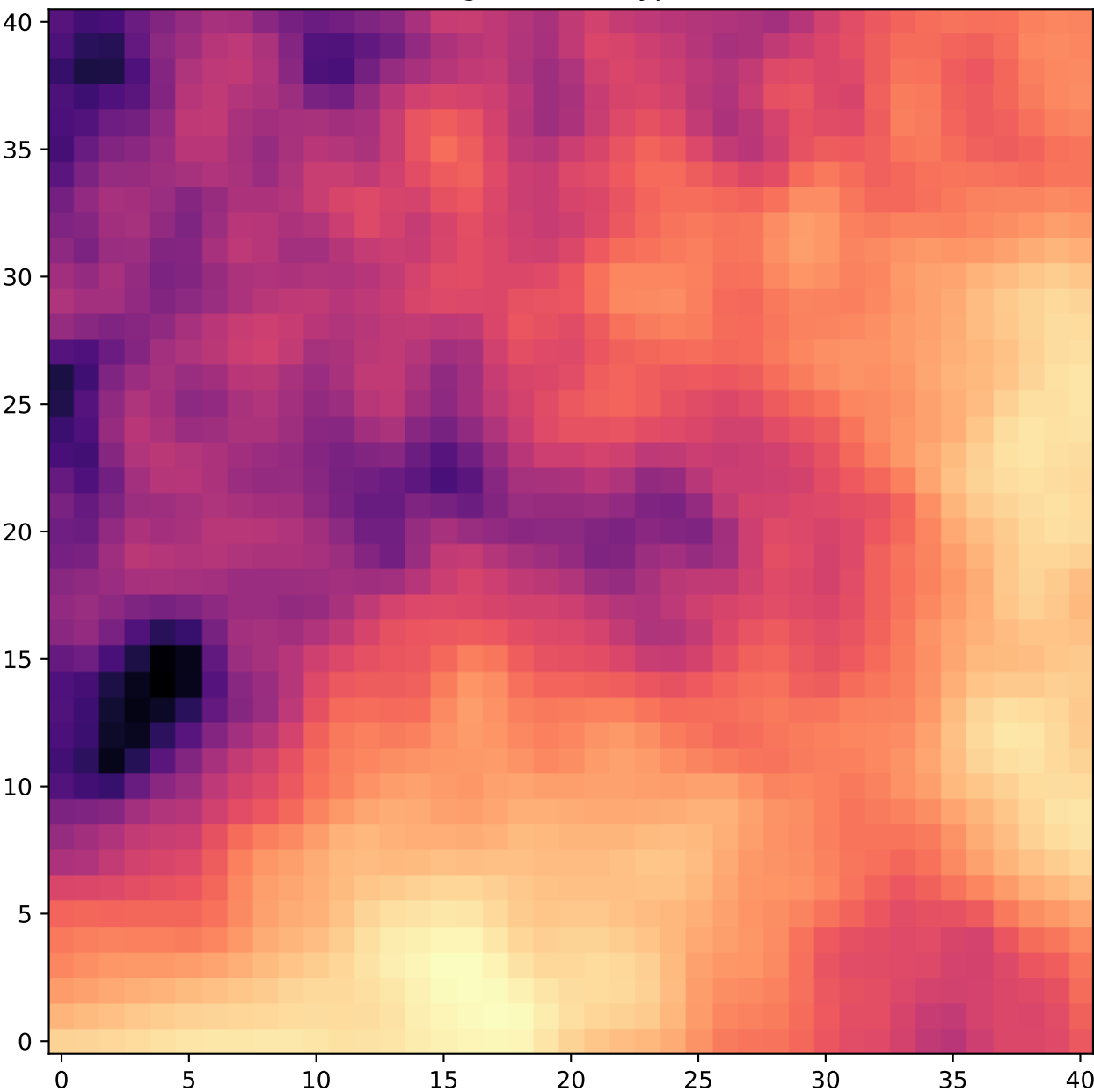
Region: 1 HI - Type 2
