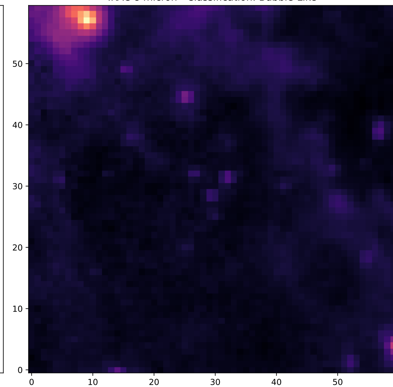
IRAC 8 micron - Classification: Bubble-Like
