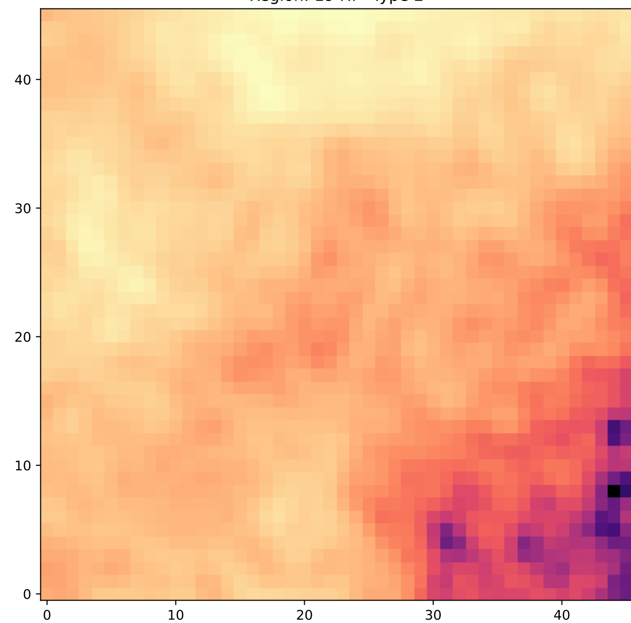
Region: 19 HI - Type 2
