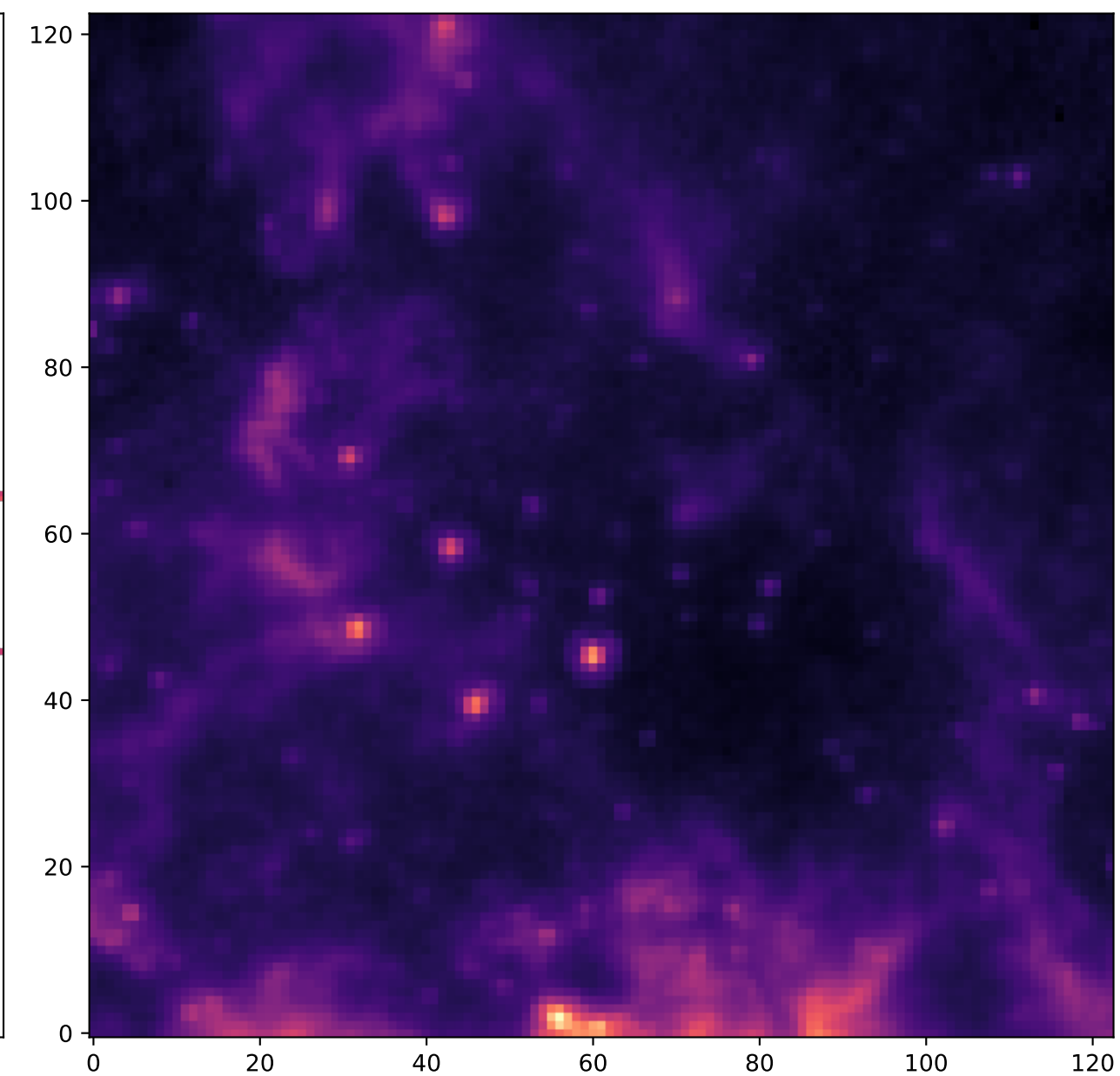
IRAC 8 micron - Classification: Diffuse
