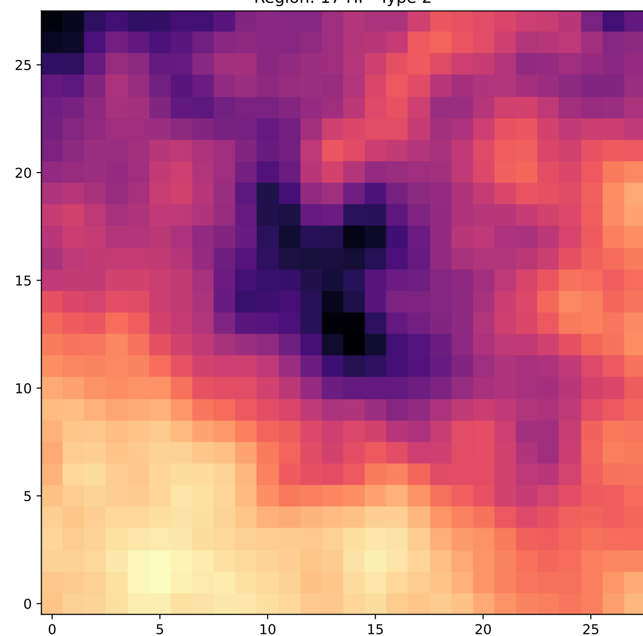
Region: 17 HI - Type 2
