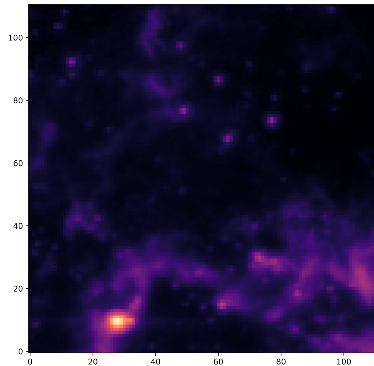
IRAC 8 micron - Classification: Bubble-Like
