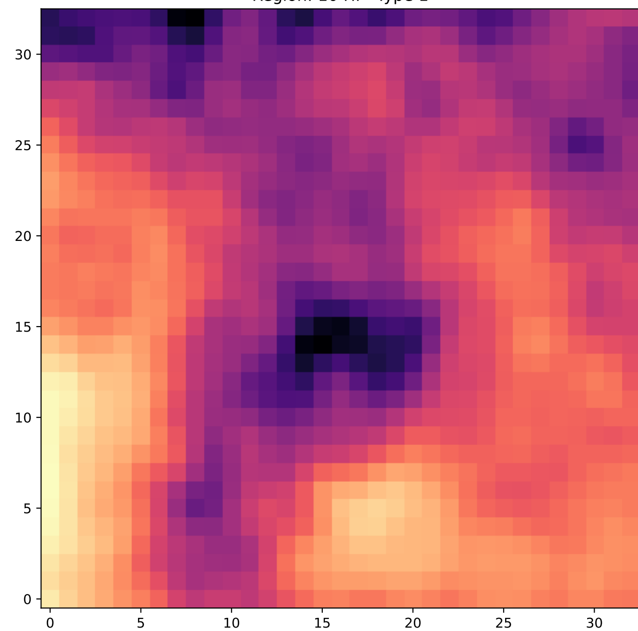
Region: 10 HI - Type 1
