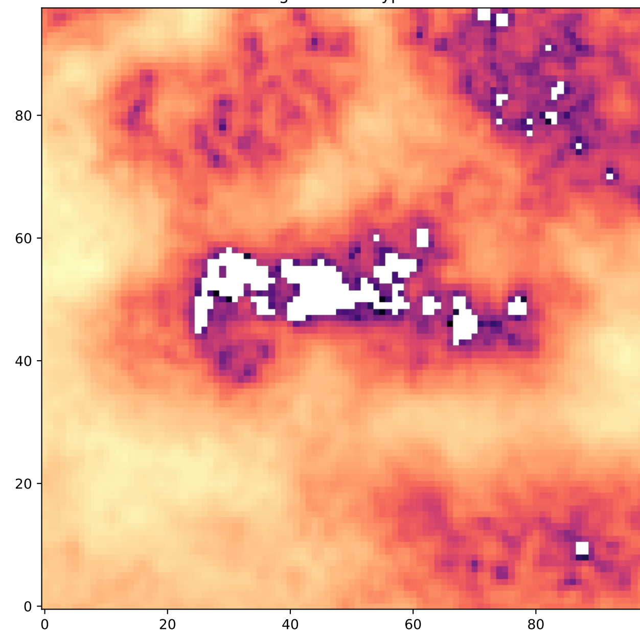
Region: 4 HI - Type 1
