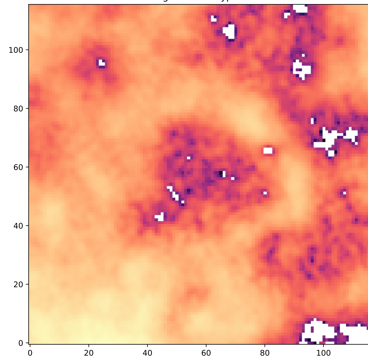
Region: 9 HI - Type 1
