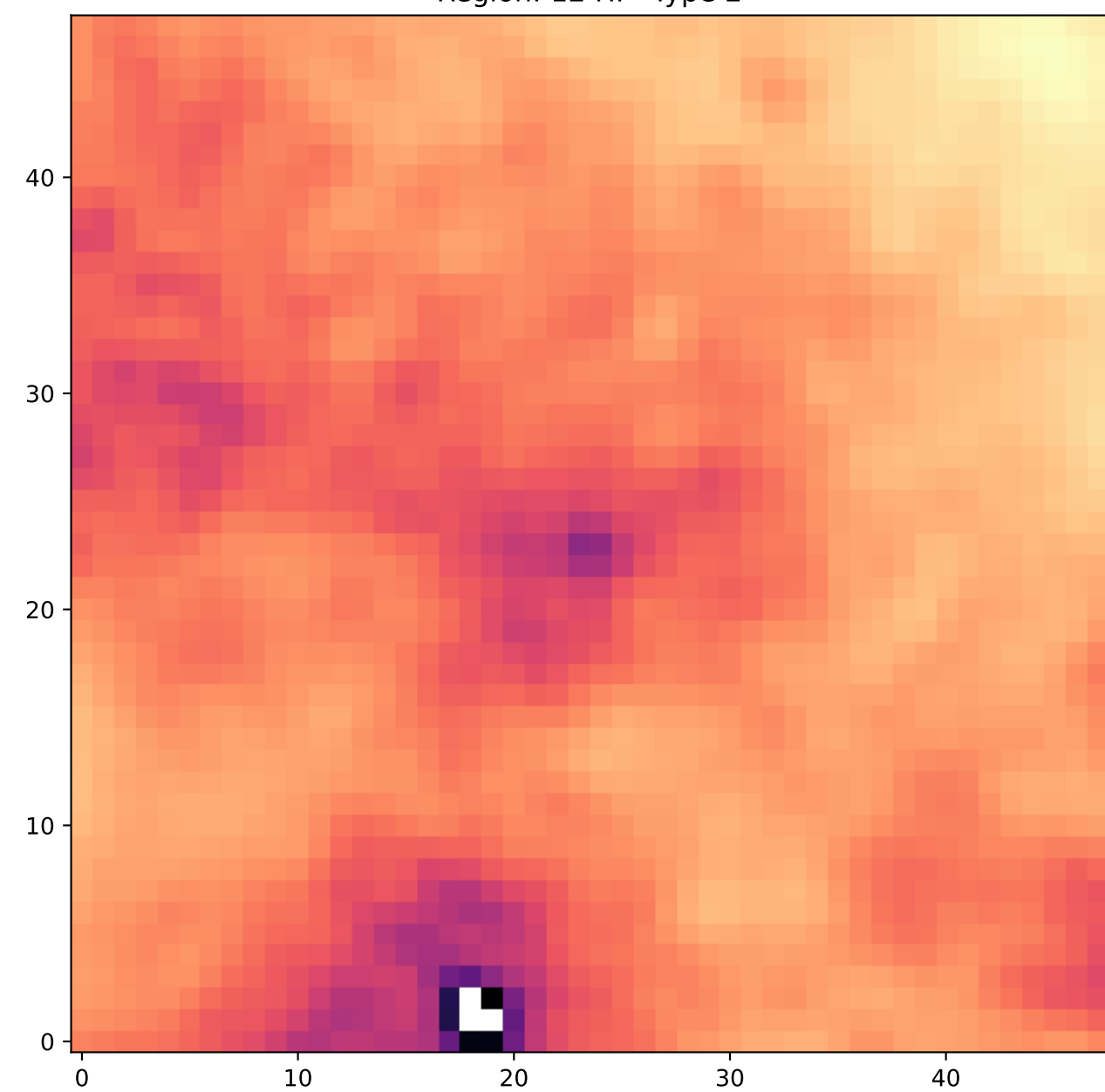
Region: 12 HI - Type 2
