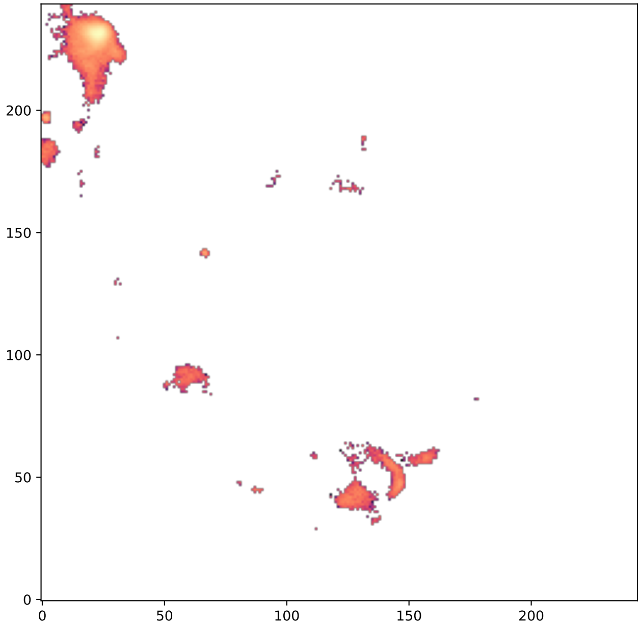
H-alpha - Classification: Diffuse
