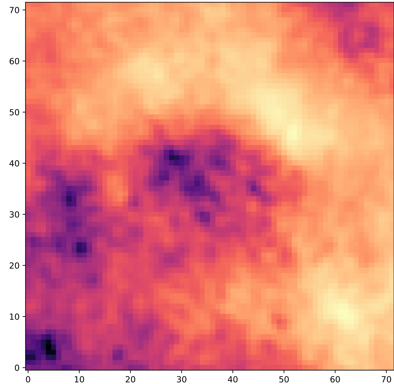
Region: 13 HI - Type 1
