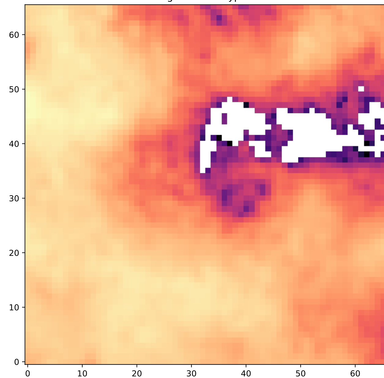
Region: 6 HI - Type 1
