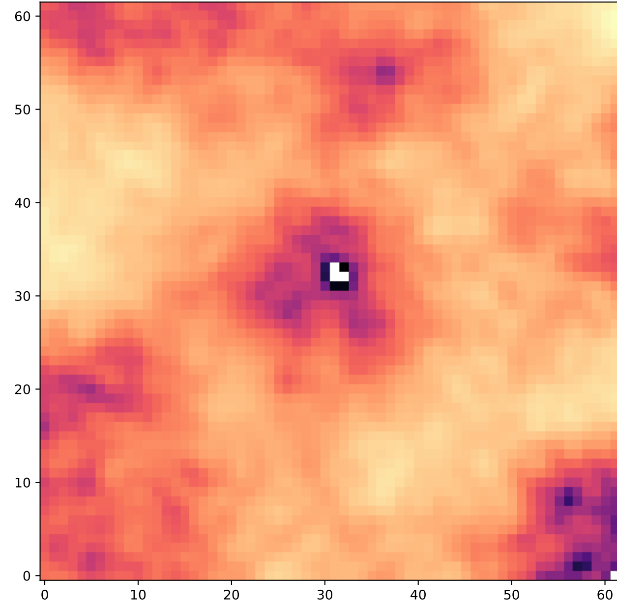
Region: 14 HI - Type 1
