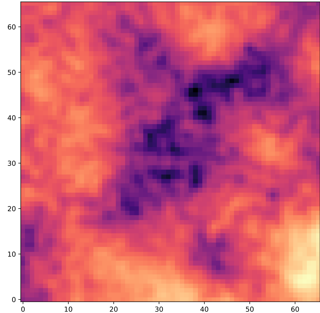
Region: 18 HI - Type 1
