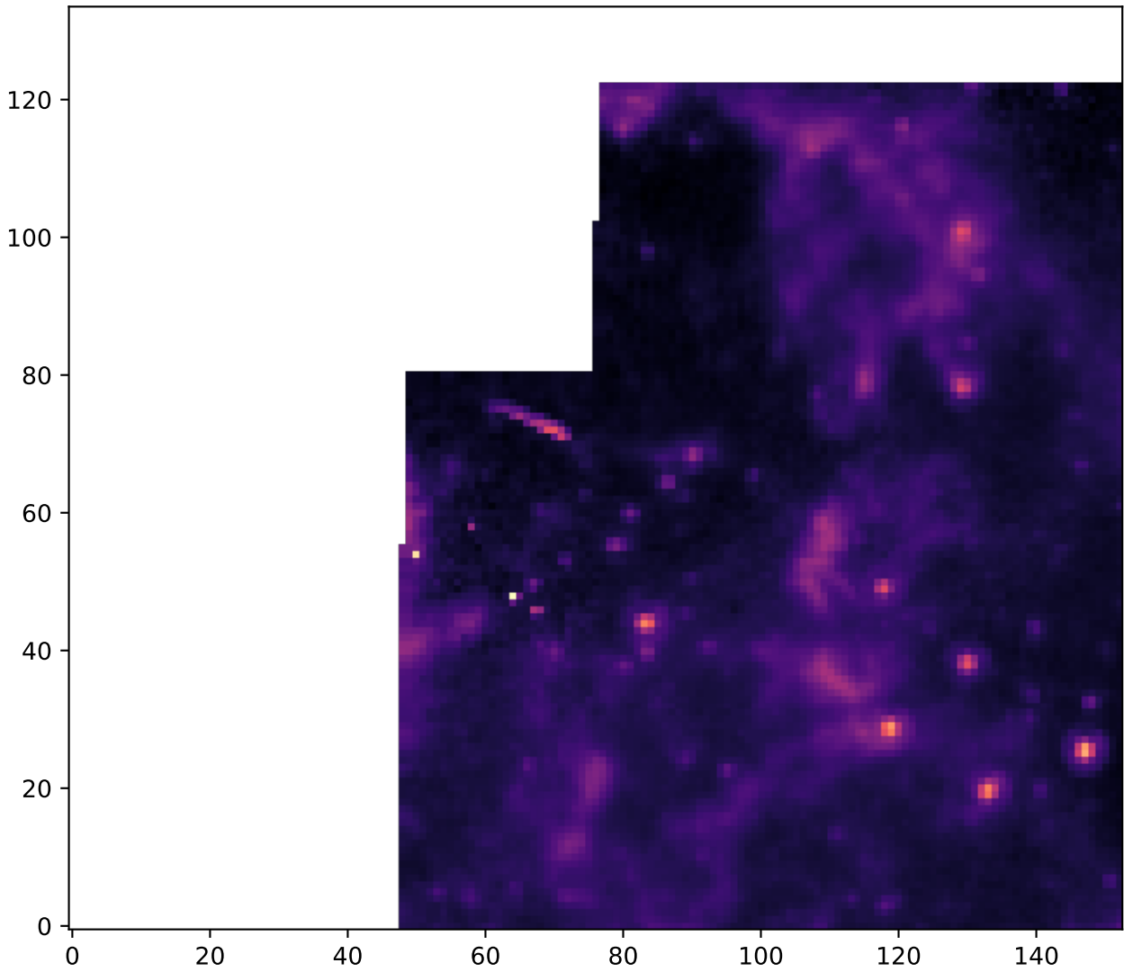
IRAC 8 micron - Classification: Diffuse
